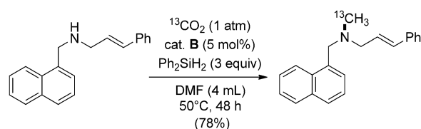
Scheme 5. Chemoselective synthesis of [\text{N-}^{13}\text{CH}_3] -naftifine using ^{13}\text{CO}_2 .
