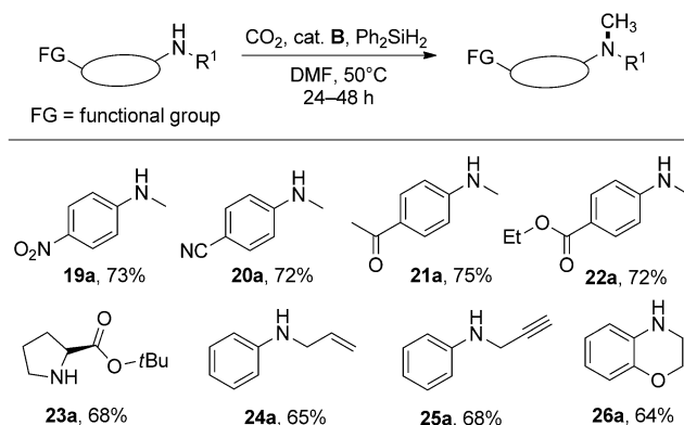
Scheme 3. Functional-group tolerance of the N-methylation of amines 19a–26a using \text{CO}_2 and \text{Ph}_2\text{SiH}_2 as the source of the methyl group. Reaction conditions: substrate (0.5 mmol), catalyst B (5 mol%), \text{Ph}_2\text{SiH}_2 (3 equiv), DMF (4 mL), \text{CO}_2 (1 atm), 50 °C, 24–48 h. Please note: shown structures are those of substrates 19a–26a , the yields are those of the corresponding N-methylated products.
