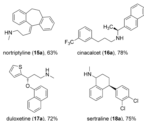
Figure 1. Pharmaceuticals 15a–18a , which were subjected to the catalytic N-methylation using \text{CO}_2 and \text{Ph}_2\text{SiH}_2 as the source for the methyl group. Please note: shown structures are those of substrates 15a–18a , the yields are those of the corresponding N-methylated products, obtained using the optimized reaction conditions (Table 1, entry 3).
